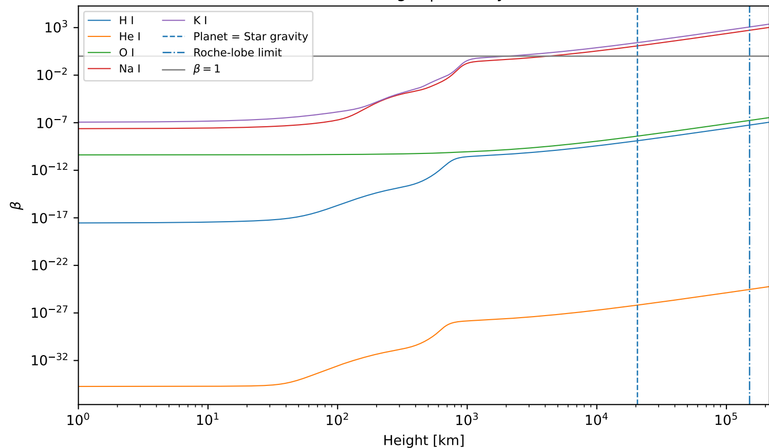
Beta vs height | Mercury-Sun
